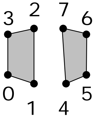
GL_QUADS
