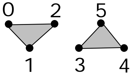
GL_TRIANGLES
