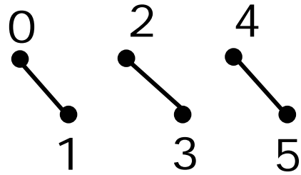
GL_LINES
