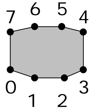
GL_POLYGON
